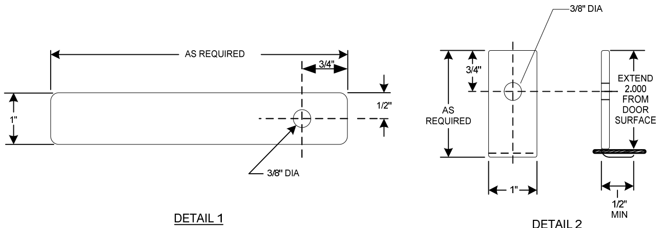
DETAIL 2
