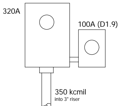
DETAIL D
