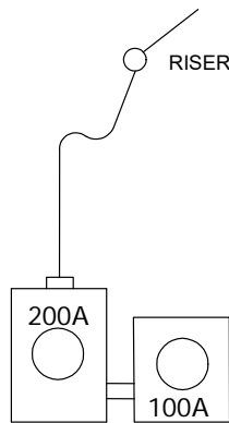
DETAIL B
