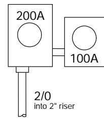
DETAIL C
