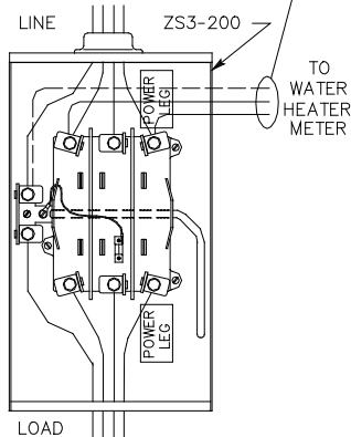
SELF-CONTAINED METER CONNECTION
