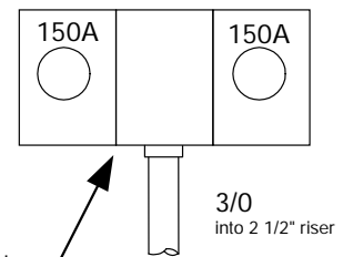
DETAIL E
