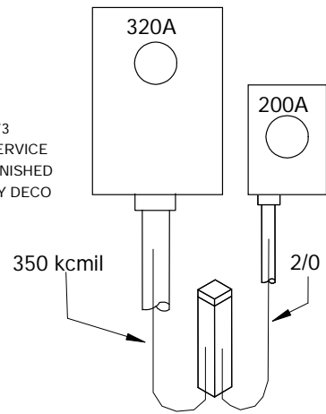
DETAIL G
