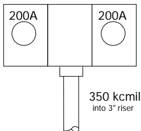
DETAIL F
