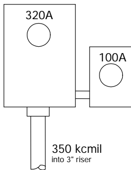
DETAIL D
