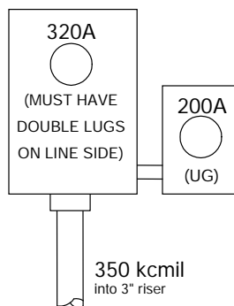
DETAIL H
